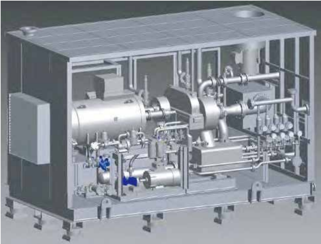
Tubo Compressor (TA-3000) - Gina Krog Project
