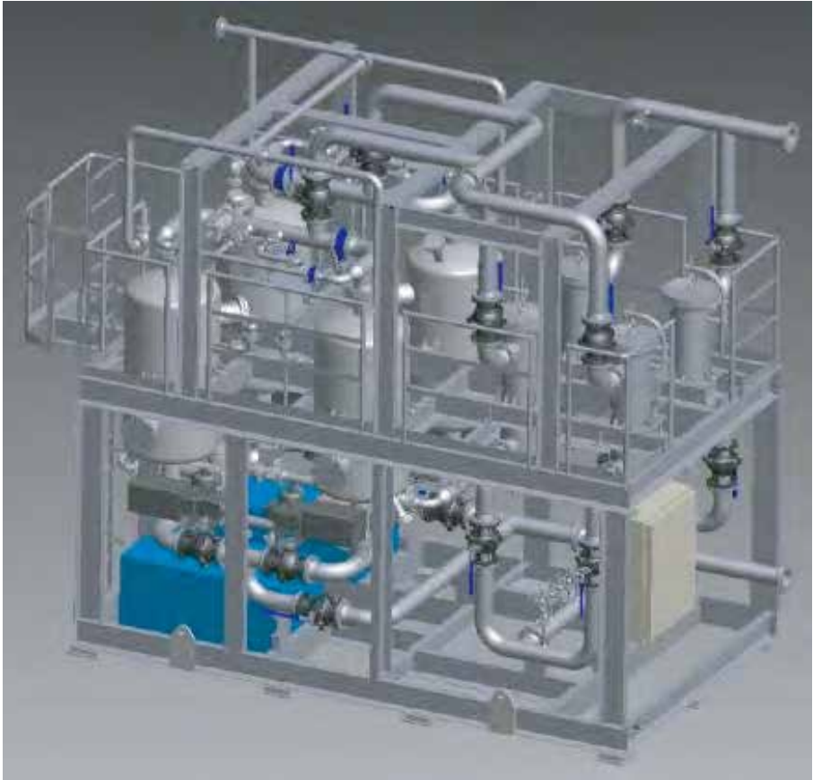
Air Dryer Package - Gina Krog Project
